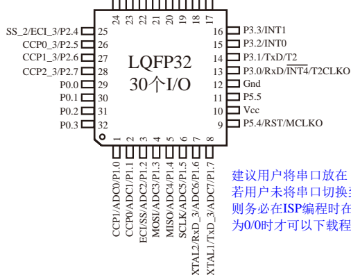
LQFP32 (9x9mm)
